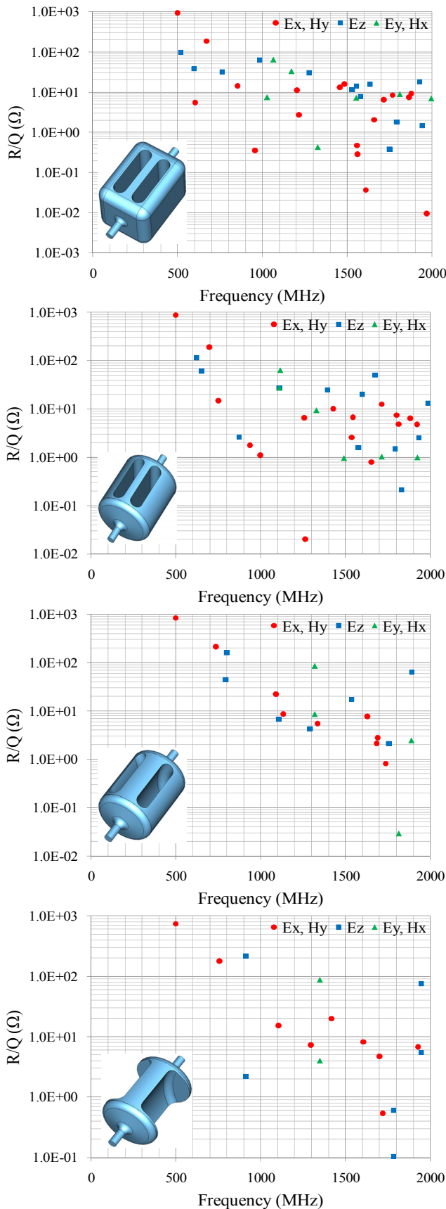
Figure 5: [R/Q] values for the rectangular shaped and cylindrical shaped parallel-bar cavities.
