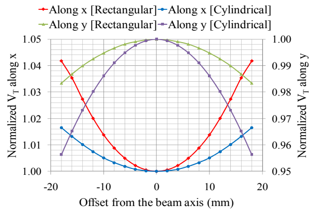
Figure 6: Normalized transverse deflecting voltage variation in x and y directions for the rectangular shaped design and cylindrical shaped design with curved bars.
