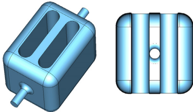
Figure 1: 499 MHz rectangular shaped superconducting parallel-bar cavity (left) and vertical cross section of the design (right).
