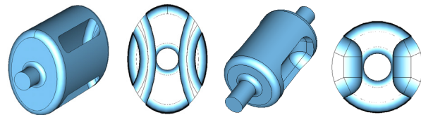
Figure 4: 400 MHz (left) and 750 MHz (right) crabbing cavities.
