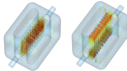
Figure 2: Electric field (left) and magnetic field (right) profiles for the rectangular shaped parallel-bar cavity.
