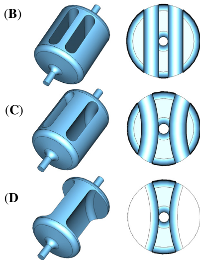
Figure 3: 499 MHz cylindrical shaped superconducting parallel-bar cavity with straight parallel bars (top), curved parallel bars (center) and bars merged to the side wall (bottom) with corresponding vertical cross sections.
