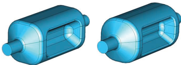
Figure 6: 400 MHz crabbing cavity with flat (left) and curved (right) inner bar surface.
