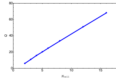
(a) Quality factor
