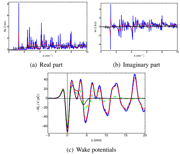
Figure 3: CSR impedance and wake potentials of the arc section in the SuperKEKB positron damping ring. The impedances and wake potentials have been normalized by the number of cells for convenience of comparison. Blue solid line: 16 cells; red dashed line: 6 cells; Green dashed line: 1 cell; Black solid line: single-bend model.
