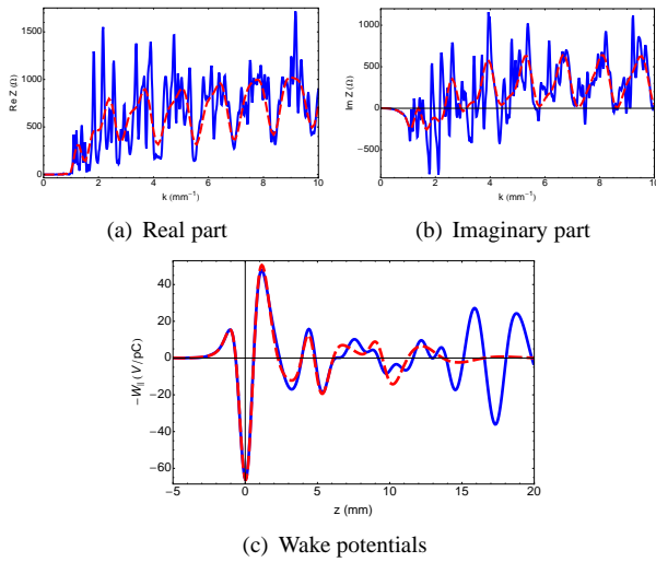
Figure 1: CSR impedance and wake potential for 4 bending magnets interleaved with equidistant drift chambers. The blue solid and red dashed lines denote the cases of with and without interference, respectively. The wake potentials have been normalized by the number of magnets. The bunch head is to the left side.
