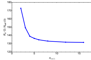
(b) Shunt impedance
