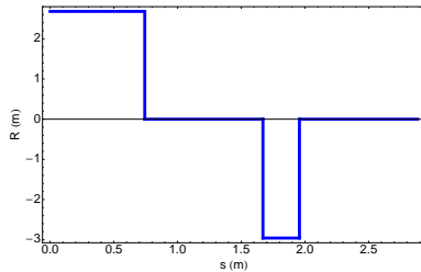
Figure 2: Bending radius as a function of orbit distance for one cell in the arc sections of SuperKEKB positron damping ring.
