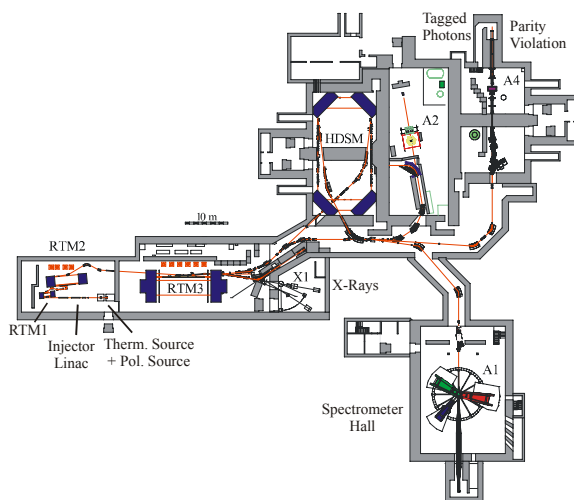
Figure 1: Floor plan of MAMI-C.
