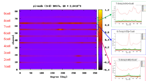
Figure 8: X-mapping result of \pi -mode of the 7 th vertical test at 9MV/m after pass-band mode measurement.
