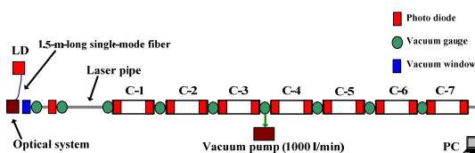
Figure 2: Schematic drawing of the experimental setup.
