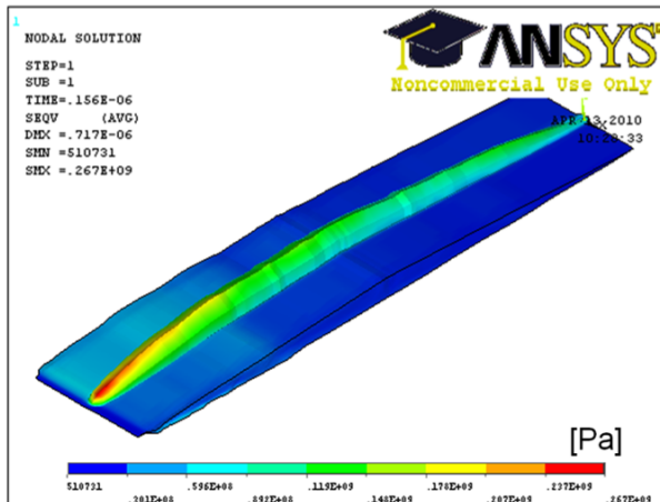
Figure 4: Equivalent stress on the spoiler body after a CLIC train hits it. The total time is one bunch train.
