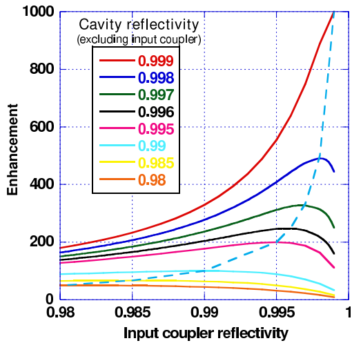
Figure 3: Enhancement as a function of input coupler reflectivity for various values of the total reflectivity of the internal cavity mirrors.
