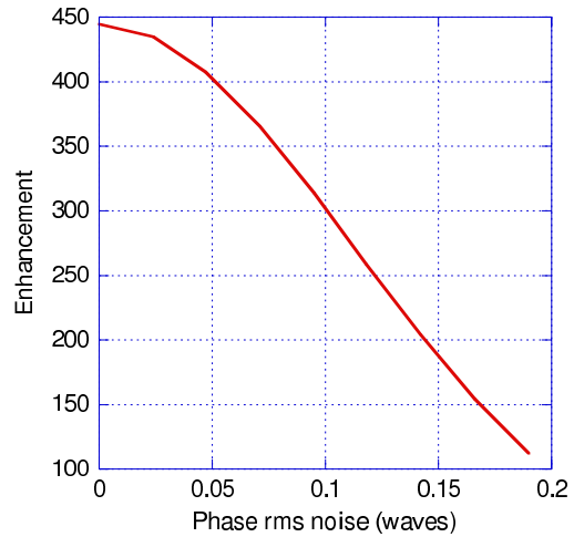
Figure 5: Cavity enhancement as a function of random phase noise in the system.
