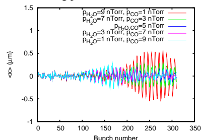
Figure 6: Snapshots of the horizontal bunch by bunch centroid, \langle x \rangle , for different compositions of the residual gas.
