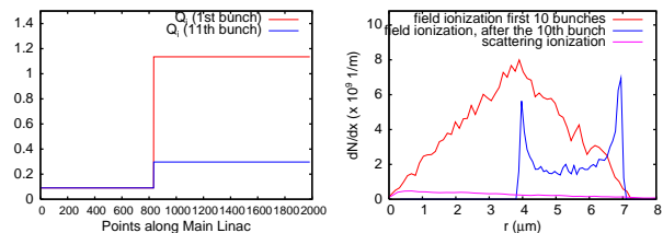
Figure 2: Left: Charges of the macro-ions produced by the first ten bunches and by the 11-th bunch as a function of the longitudinal position along the Main Linac (in non-uniform steps). Right: distributions of the ions at the time of their production, red: field ions, first 10 bunches; blue: additional field ions produced by each bunch from 11th to 312th; purple: scattering ions.
