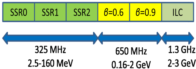
Figure 4: Accelerating module configuration of the 3 GeV CW linac in IC-2.
