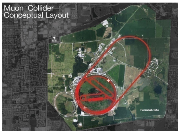
Figure 6: Conceptual layout of a Muon Collider. The Project X linac is situated on the lower half of the Tevatron infield, upstream of the rings needed to prepare the linac beam for targeting.
