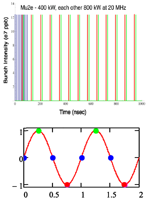
Figure 3: Illustration of the utilization of the 2.5 MeV chopper and 3 GeV separator to provide a particular bunch pattern. Top: the loading of 325 MHz buckets to support three distinct experimental users. Bottom: The arrival times of the various buckets at the deflecting mode separator cavity.
