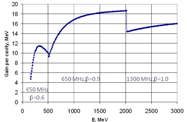
Figure 5: Energy gain per cavity through the CW linac portion of Project X, IC-2
