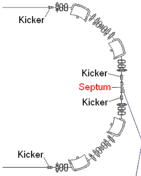
Figure 1: Schematic of 1/2 MLS storage ring with injection
