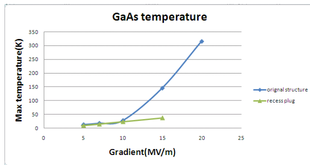
Figure 5: The GaAs crystal temperature simulation with two kind of plug designing.
