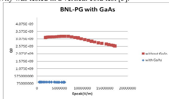
Figure 2: Quality factor vs. gradient with and without GaAs cathode at 2k.
