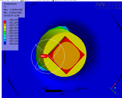
Figure 4: Temperature distribution at 5 MV/m, calculated with ANSYS. The picture shows the cavity walls (blue), the tip of the plug (yellow) and the GaAs crystal (orange/red).
