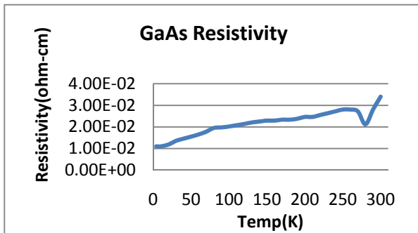
Figure 3: The GaAs resistivity by the temperature from 300K to 4K.
