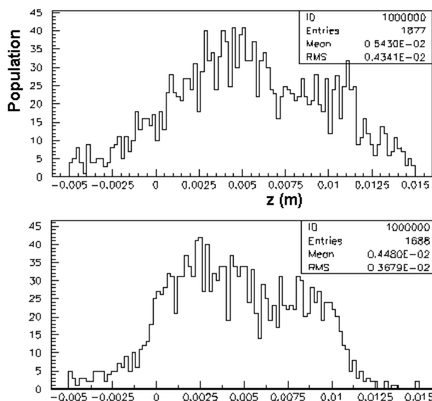
Figure 5: Longitudinal distribution at the exit of the first tank in the case of deceleration approach for the 1.428 GHz scenario (top) and the TM020 approach (bottom).
