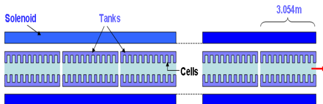
Figure 3: The 2.856 GHz 3.054m long tanks after the AMD encapsulated in a 0.5 T solenoid field.
