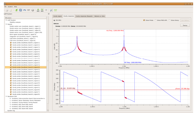
Figure 5: Characterization of RF system in GUI as part of Libera LLRF RF system diagnostics functionality.
