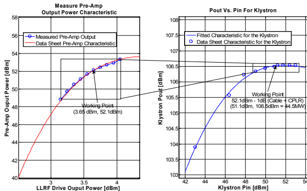
Figure 8: Pre-amp and klystron output power dependence measurements.
