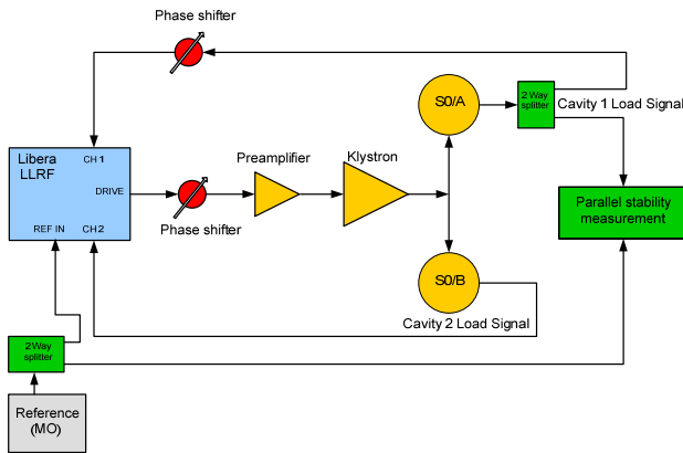
Figure 7: Measurement set-up.
