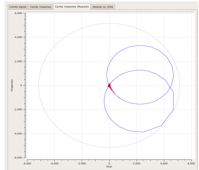
Figure 6: Nyquist stability analysis of the control system.
