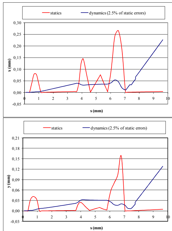
Figure 5: Comparison of the effect of static and dynamic errors on trajectory deviation
