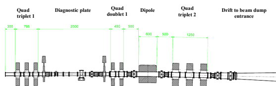
Figure 1: HEBT line projection on yz plane
