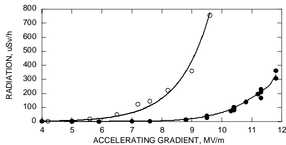
Figure 2: Linac cavity radiation levels pre- (open circles) and post- (full circles) helium processing.
