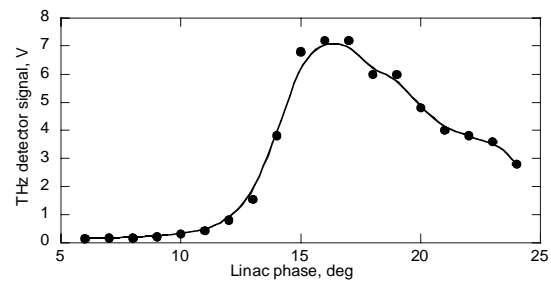
Figure 4: Intensity of the terahertz beam on its axis as a function of the linac off-crest phase.
