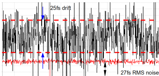
Figure 6: Operation at 20pC showing 27fs RMS noise and 25fs drift over 3 hours.
