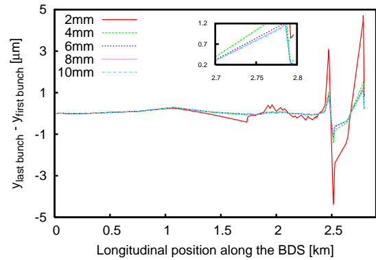
(a) 3 TeV
