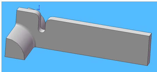
Figure 2: XL5 Output coupling cell and iris (¼ geometry).
