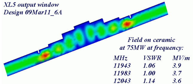
Figure 5: Fields in XL5 Output window, axial symmetry.
