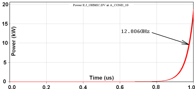
Figure 6: XL5 MAGIC simulation of unloaded output structure shows oscillation after 600ns at 12.806GHz.
