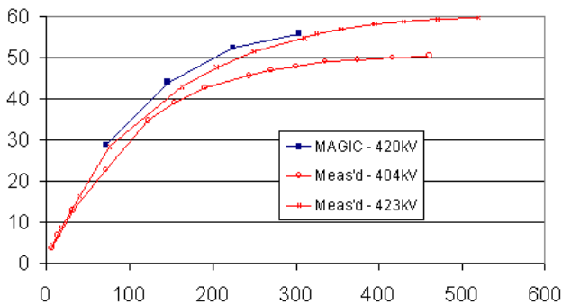
Figure 3: XL5 MW output vs. W input for simulation at 420kV and XL5-1 test data at 404kV and 423kV.
