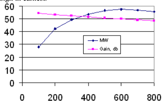
Figure 1: A 1.5D simulation of output power and gain vs. rf drive at V_b=400\text{kV} .
