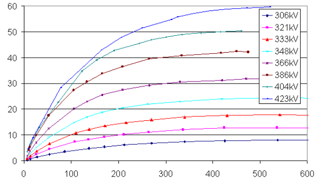
Figure 8: Gain curves for the XL5-1.
