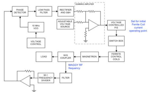
Figure 9: Feedback Circuit
