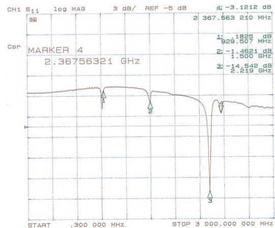
Figure 6: Frequency sweep with two YIG rods with a magnetic field 53% of the YIG saturation magnetization.
