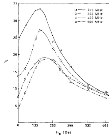
Figure 5: Re(\mu) for Mg_{.35}Zn_{.65}Fe_2O_4 magnesium-zinc spinel ferrite [6].
