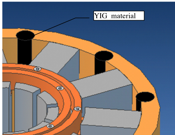
Figure 1. Schematic drawing of the strapped anode structure showing the location of the YIG rods
