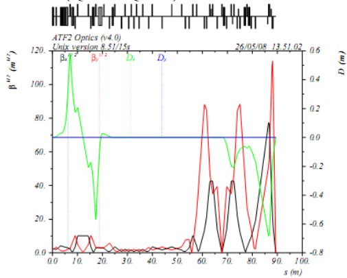
Figure 3: Twiss parameter of the ATF2 line
