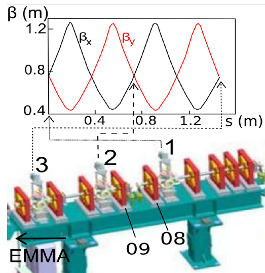
Figure 1: Matching and tomography sections of the injection line to EMMA, showing design \beta -functions at the three screens.
