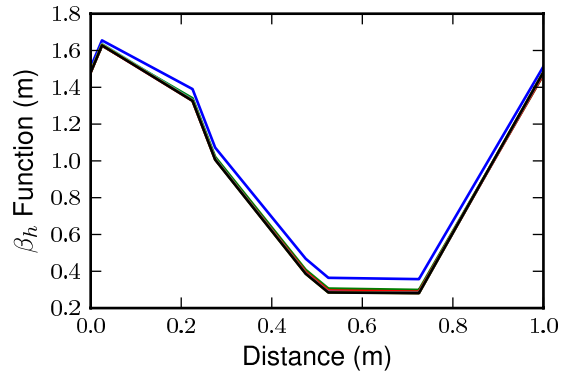
Figure 5: Beta functions at 100 mm mrad
