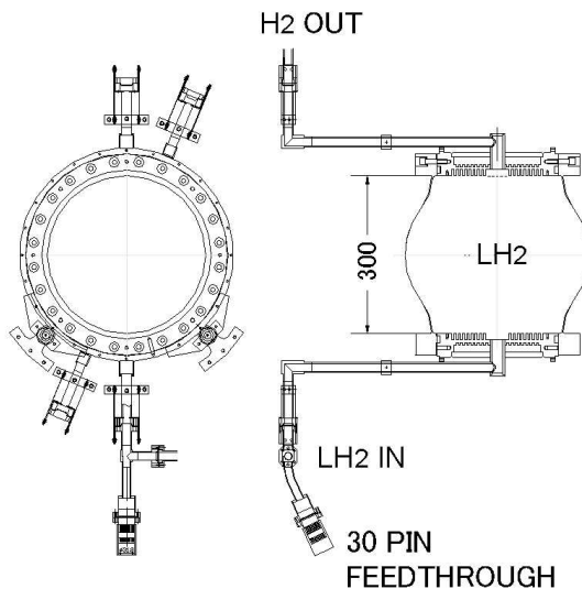
Figure 2: MICE liquid hydrogen absorber.
