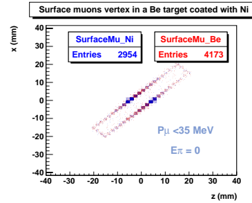
Figure 8: Distribution of surface muon vertex in a Be target coated with Ni.
