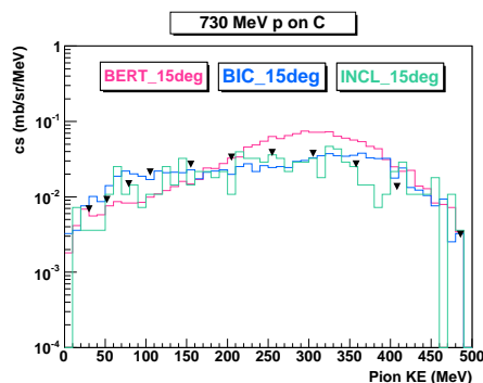
Figure 1: Double differential cross section for positive pion production at 15 degrees with respect to the proton beam.
