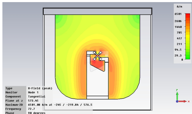
Figure 2: Magnetic field in the cross section of the ReA3 cavity.
