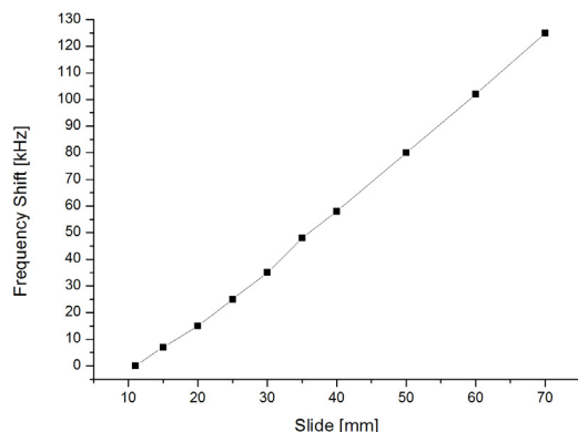
Figure 6: Frequency range of the tuners.
