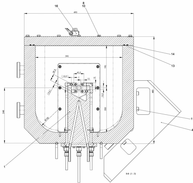
Figure 3: Scheme of the ReA3-RFQ with a square cross section and a sight of a stem and its cooling system.
