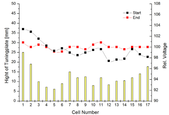
Figure 5: Relative longitudinal voltage distribution before (black) and after (red) the tuning. The bars show the positions of the tuning plates.
