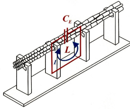
Figure 4: Basic cell of the 4-rod RFQ structure.
