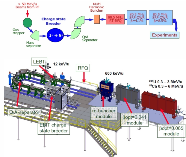
Figure 1: Overview of the Reaccelerator Facility Setup of the ReA3 at MSU [1].
