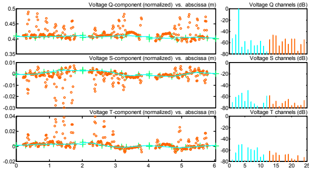
Figure 4: RFQ 3 tuning after last 5 th iteration.
