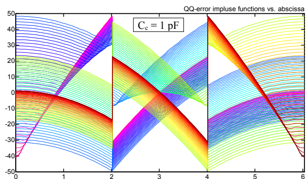
Figure 2: h_{QQ} vs. z (abscissa) and z_0 (color code), RFQ 3 .
