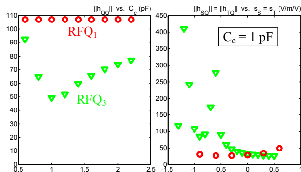
Figure 1: Stability analysis of RFQ 1 and RFQ 3 .
