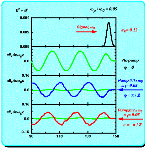
Figure 1: Top to bottom: (i) single short laser pulse with a_0 = 0.12 and frequency \omega_0 propagates from left to right; (ii) short pulse generates a weak plasma wake E_x ; (iii) in the presence of counter-propagating pump with a_1 = 0.05 and frequency \omega_1 = 1.1\omega_0 the wake is enhanced, and its phase is shifted by \pi/2 with respect to the “regular” wake of (ii), which is also shown for comparison; (iv) Same as (iii), only a down-shifted pump with \omega_1 = 0.9\omega_0 is used, and the phase shift is -\pi/2 .
