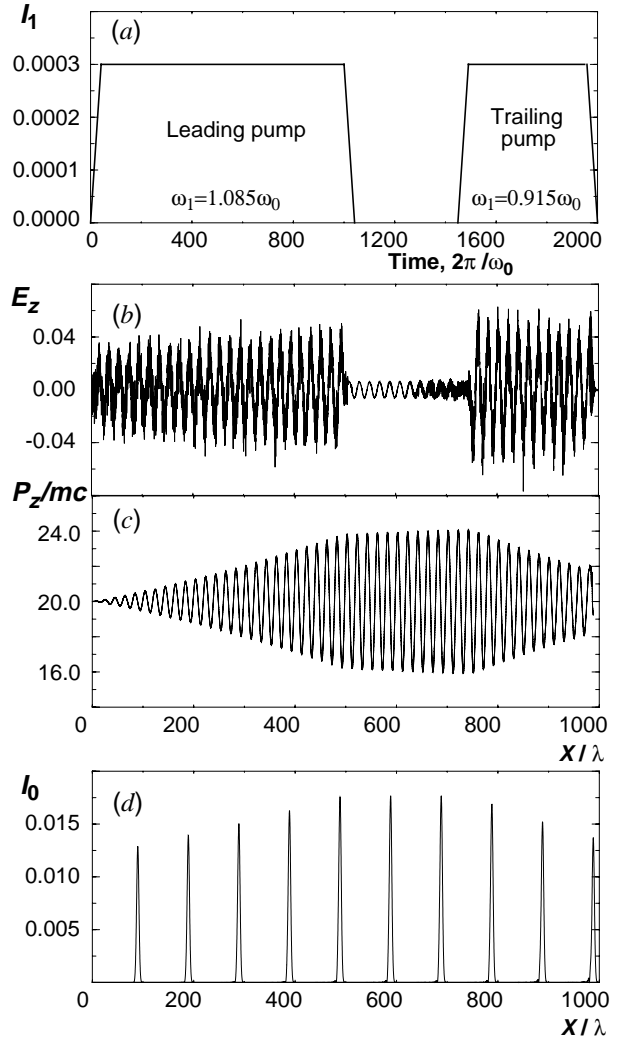
Figure 2: Collision between a short timing beam ( a_0 = 0.08 , \tau_L = \omega_p^{-1} ) and an intermittent pump ( a_1 = 0.012 ) in n_0 = 2.5 \times 10^{18} \text{cm}^{-3} plasma ( \omega_0/\omega_p = 20 ). 10 MeV electrons are continuously injected into the plasma. (a) Time-dependence of the pumping beam intensity I_1 = 2a_1^2 ; (b) longitudinal electric field eE_z/mc\omega_p ; (c) propagation of the TB through the plasma, I_0 = 2a_0^2 ; (d) phase space of injected electrons.
