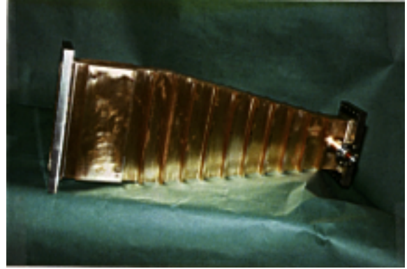
Figure 5: HOM Waveguide Transition.
