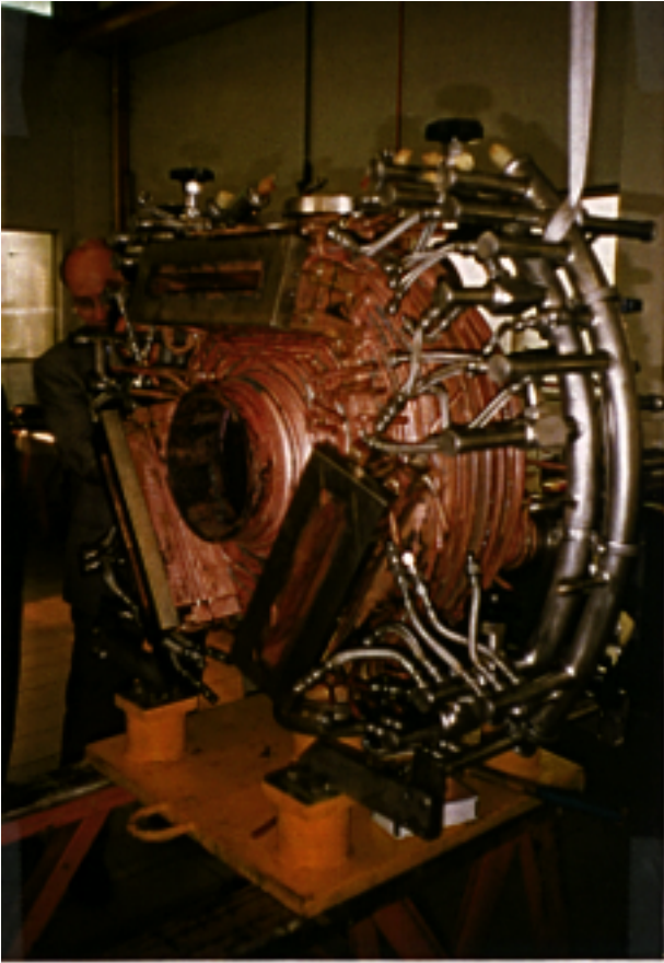
Figure 4: DAΦNE RF Cavity during fabrication at Zanon.
