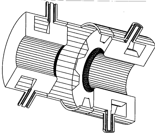
Figure 6: CAD view of the overdamped kicker cavity.
