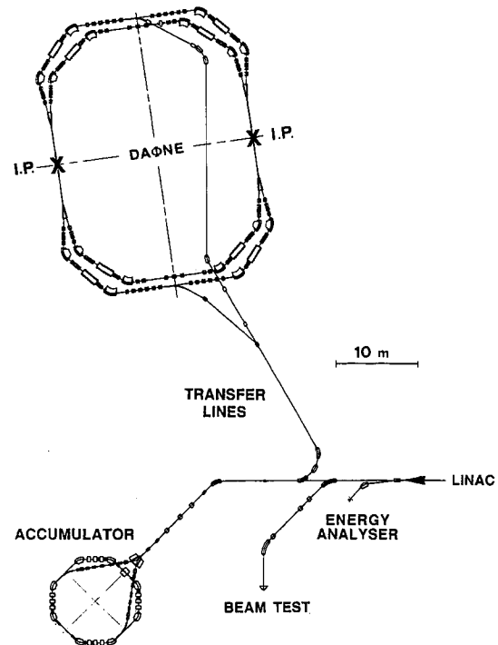
Figure 1: Layout of DAΦNE and its injector.
