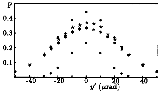
Figure 2. F(y') scan for x'=0 . Ideal crystal: (o) first-pass and (●) overall efficiencies. Imperfect crystal: overall efficiency with t=1 \mu\text{m} (*) and t=50 \mu\text{m} (x).
