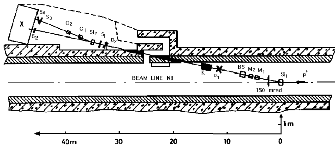
Figure. 1. The scheme of crystal beam line and experimental setup: Si_1, Si_2 – deflecting and testing crystals, M_1, M_2 – corrector magnets, BS – beam stopper, D_1, D_2 – proportional chambers, K – collimator, S_1 - S_4 – scintillator counts, C1, C2 – microstrip detector stations, X – beam absorber.
