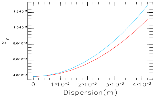
Figure 2: The vertical emittance as a function of the external dispersion. The blue line is the effective emittance, and the red line is the vertical emittance \epsilon_{y,0} .
