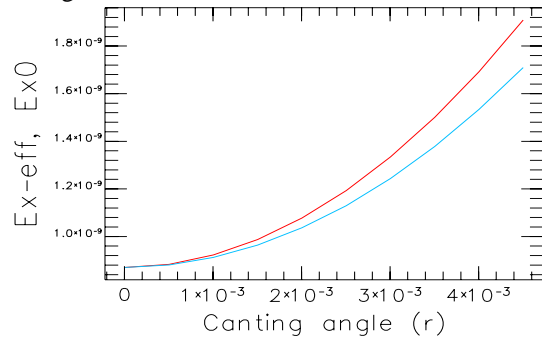
Figure 3: The natural and effective horizontal emittance as functions of the canting angle.
