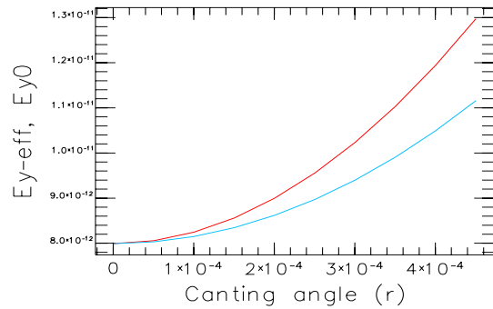
Figure 4: The equilibrium and effective vertical emittance as functions of the canting angle.
