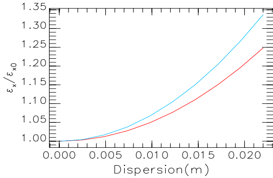
Figure 1: The horizontal emittance growth ratio as a function of external dispersion in the straights. The blue line is for the effective emittance, and the red line is for the horizontal emittance \epsilon_{x,0} .
