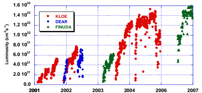
Figure 1: DAΦNE peak luminosity for KLOE (red), DEAR (blue) and FINUDA (green).
