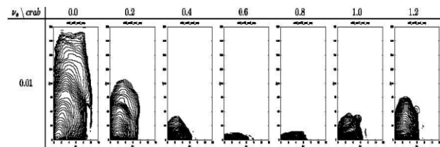
Figure 3: Distribution tails vs crabbing sextupole intensity.
