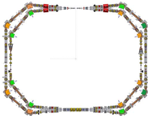
Figure 5: Upgraded DAΦNE layout.
