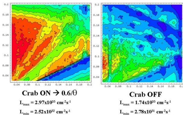
Figure 2: Luminosity vs tunes scan. CW ON, 0.6/\theta (left). CW OFF (right).
