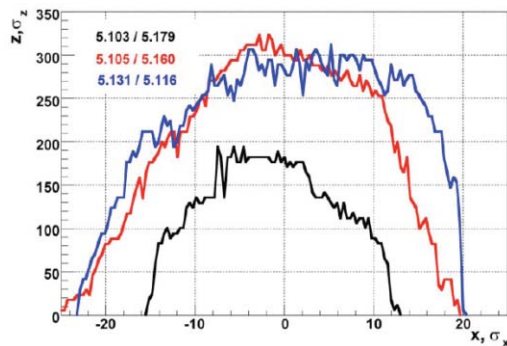
Figure 4 - Optimized DA for different working points.
