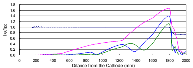
Figure 1: Simulation of the RF interaction. Lines show modulated RF currents of the corresponding cavity modes.
