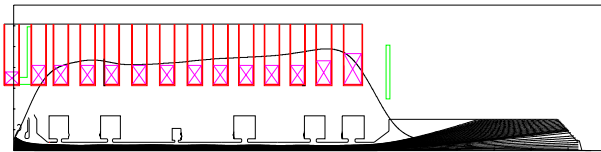
Figure 5: Focusing magnet and beam transport.
