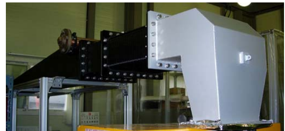
Figure 12: Waveguide and 1 MW CW RF dummy load.
