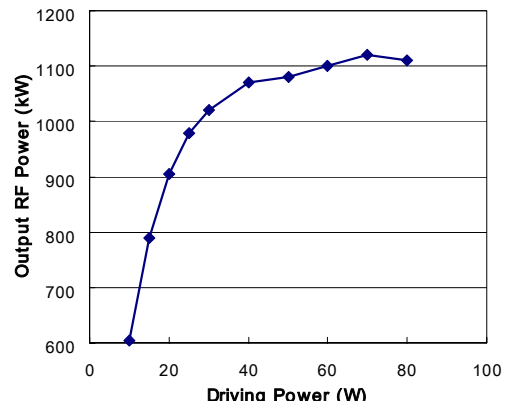
Figure 3: Transfer curve at Q_{ex}=55 .
