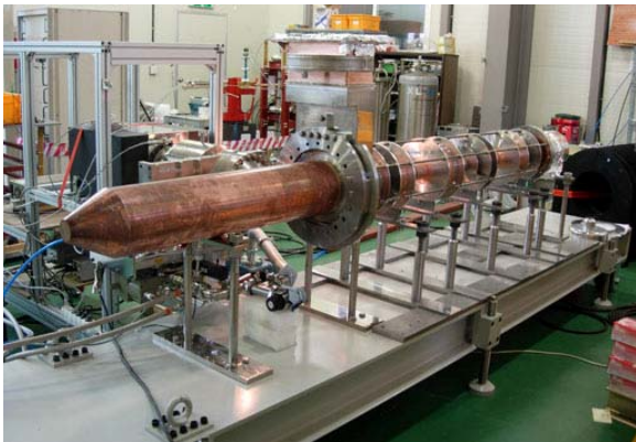
Figure 10: 700 MHz PEFP prototype klystron tube after the final welding.
