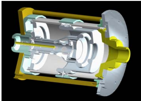
Figure 4: Electron gun.
