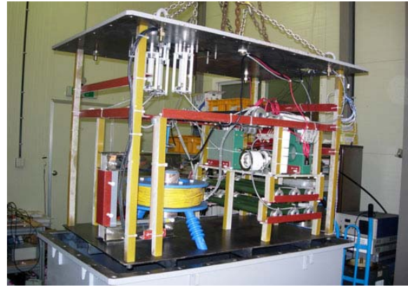
Figure 11: Cathode heating and pulse power system.
