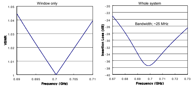
Figure 7: RF characteristics of the RF output circuit.
