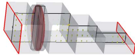
Cascade Step WG Transformer
