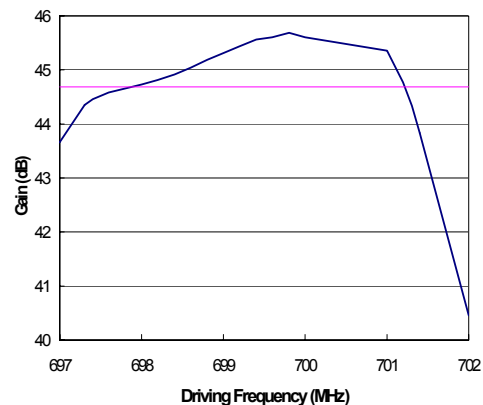
Figure 2: RF gain characteristics.
