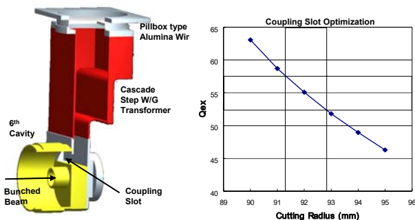
Figure 6: Schematics of the RF output circuit and dependencies of Q ex on the size of the coupling slot.
