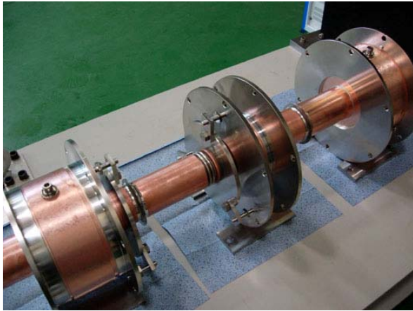
Figure 9: Cavities before the final welding.
