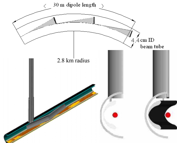
Figure 5. Photon stop in dipole: a) placement along dipole; b) cutaway view; end view at c) injection; d) collision.
