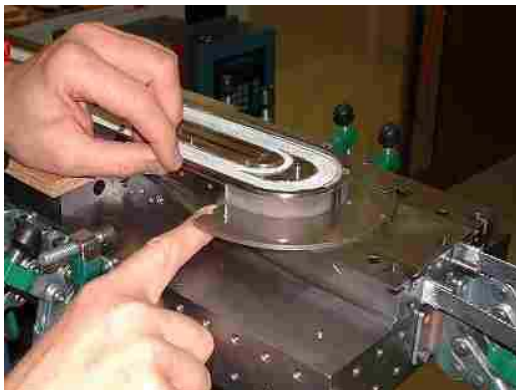
Figure 3. Applying laminar springs, ribs and plates to inner winding of \text{Nb}_3\text{Sn} .
