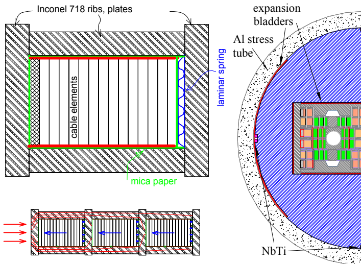
Figure 2. Stress management in a block coil geometry.
