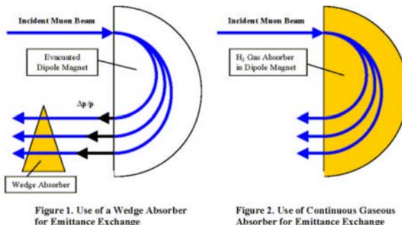
Figure 8: Conceptual drawing of emittance exchange with a homogeneous absorber (right) compared with conventional emittance exchange (left).
