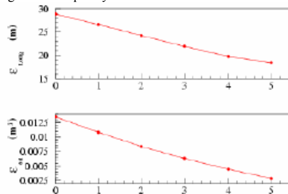
Figure 9: Simulated MANX cooling of normalized longitudinal and 6D emittances in a 5 m long HCC filled with liquid hydrogen.
