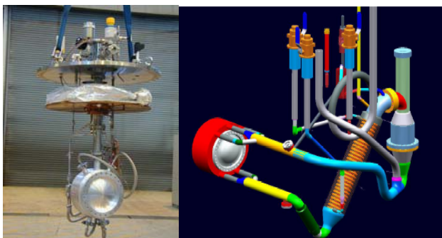
Figure 4: Two LH 2 absorber prototypes, convection type, internal heat exchange (left) and forced-flow, external heat exchange (right).
