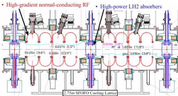
Figure 2: Cooling channel from Neutrino Factory Study II.
