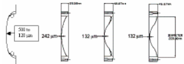
Figure 5: Evolution of thin window profiles. From left to right: standard torispherical shell with tapered ends to a normal surface, tapered torispherical to flange, inflected to flange, and thinned inflected.
