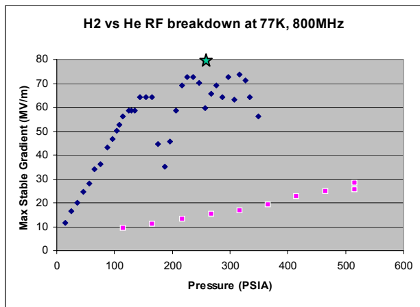
Figure 7: Paschen curve measurements for hydrogen (diamonds) and helium (squares). After a period of conditioning, a maximum gradient of 80MV/m was achieved (star) in GH 2 .
