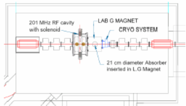
Figure 3: Plan view of a complete cooling cell test at the MTA.
