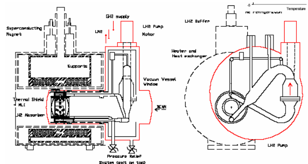
Figure 6: LH 2 forced-flow, external heat exchange prototype, shown inside a cryostat, inserted into the bore of the MTA solenoidal magnet sideview(left) and beam view (right).
