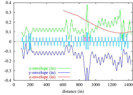
Figure 3: Calculated beam envelope size (inches) at 800 \mu\text{A} , showing transverse growth due to decreasing bunch length. The red line represents the bunch length divided by 20.
