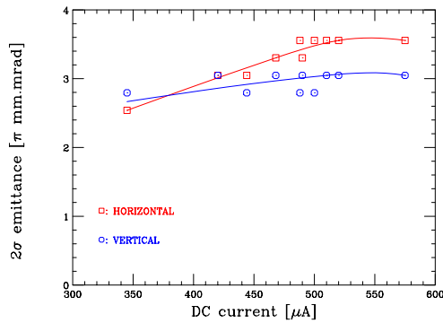
Figure 2: Fitted beam emittance ( 2\sigma ) vs. current.
