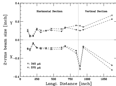
Figure 1: The beam sizes ( 2\sigma ) at dc currents 345 and 575 \mu\text{A} . The data points are the measurements. The dashed line is only meant to guide the eye.
