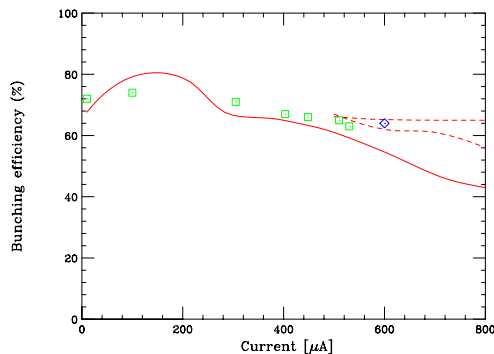
Figure 5: Bunching efficiency vs. beam current. The data points are the machine operational results: the 'diamond' was achieved with \sim 50^\circ phase acceptance due to an increased rf voltage. The solid line is the calculation result with 36^\circ cyclotron phase acceptance. The lower dashed line is the calculation result for a 50^\circ phase acceptance with the present buncher system; the upper dashed line is the calculated performance for the 36^\circ phase acceptance but with the third buncher added.
