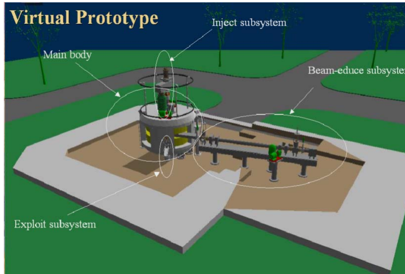
Figure 2: Virtual Prototype of CYCIAE-30 Created by AVPS
