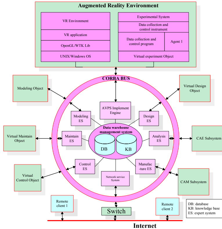
Figure 1: Framework of AVPS
