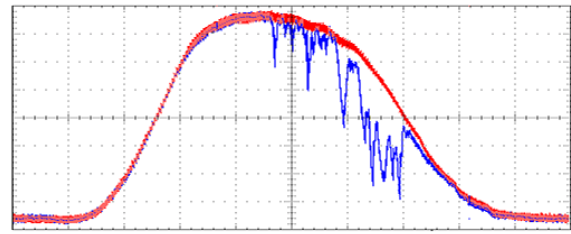
Figure 3: Ring filling patterns: The abscissa extends over 1 \mu\text{s} , i.e. approx. one revolution, showing the 480 buckets. Half of the ring had been filled initially to 200 mA (red) at high chromaticities of +5 . When lowering the vertical chromaticity to zero, single bunches or complete sections from the bunch train's tail region are lost suddenly, leaving the eroded pattern (blue) within a few minutes.
