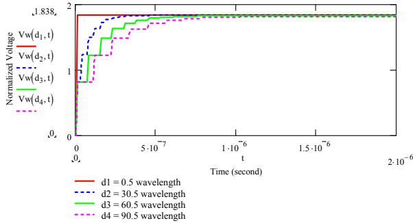
Figure 3 – Peak standing wave voltage vs. time in the transmission line for a reactively tuned case with a detuning \Delta f = BW where BW = f_0/Q
