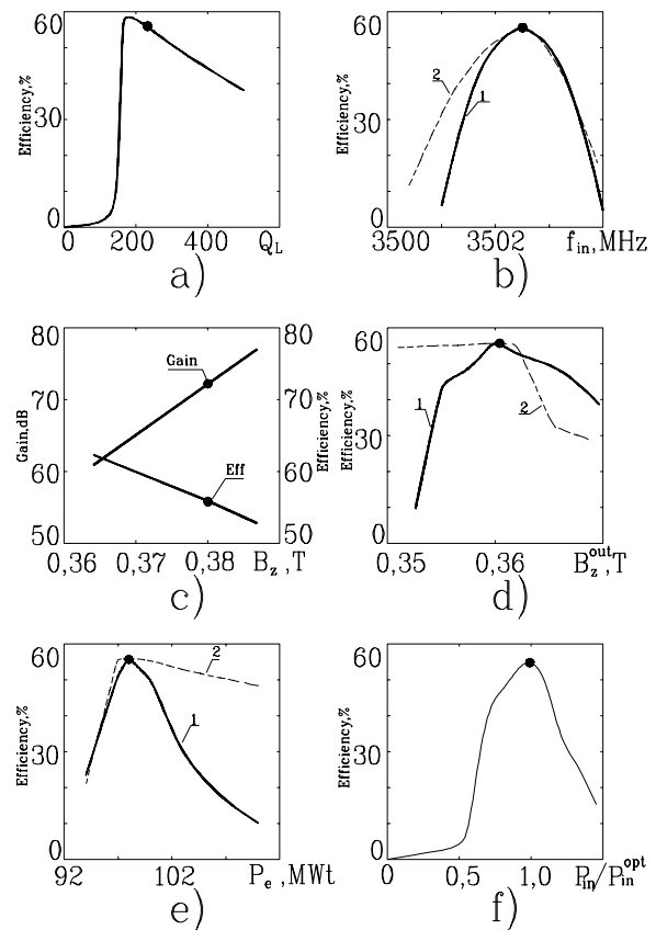
Figure 3: Experimental and calculated curves: a) loading dependence; b) input frequency dependence; c) DC magnetic field dependence of gain and efficiency; d) output cavity DC magnetic field dependence of efficiency; e) beam power dependence of efficiency; f) efficiency versus drive power. 1 corresponds to experimental data, 2 — to simulation results.
