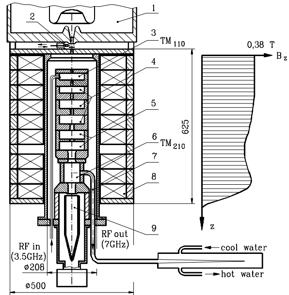
Figure 1: Schematic layout of the magnicon: 1 – electron source; 2 – vacuum valve; 3 – drive cavity; 4 – gain cavities; 5 – penultimate cavity; 6 – output cavity; 7 – waveguide ( \times 2 ); 8 – solenoid; 9 – collector.
