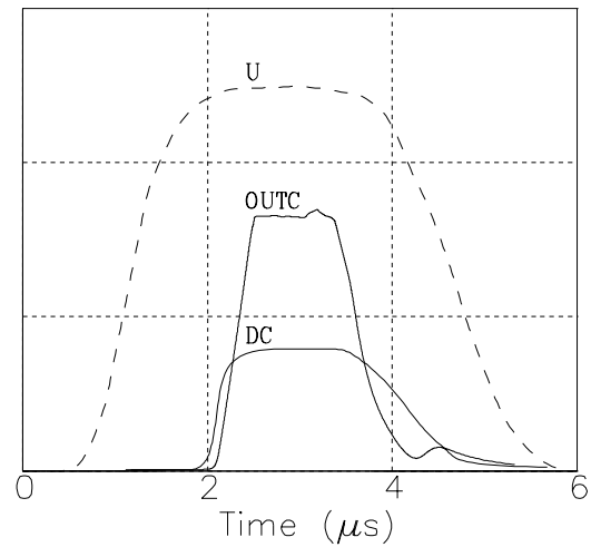
Figure 2: Oscillograms: U — beam voltage; DC — drive cavity signal; OUTC — output cavity signal.
