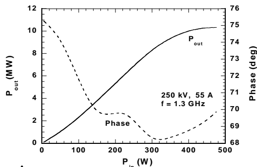
Figure 6: Output power and phase vs input power
