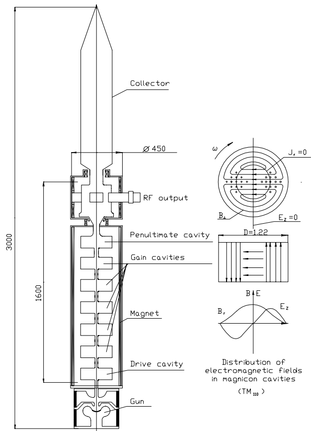
Figure 1: Schematic of a magnicon amplifier
