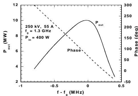
Figure 5: Output power and phase vs f-f_0
