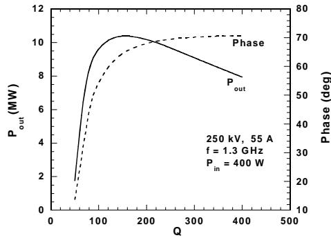
Figure 4: Output power and phase vs Q of output cavity
