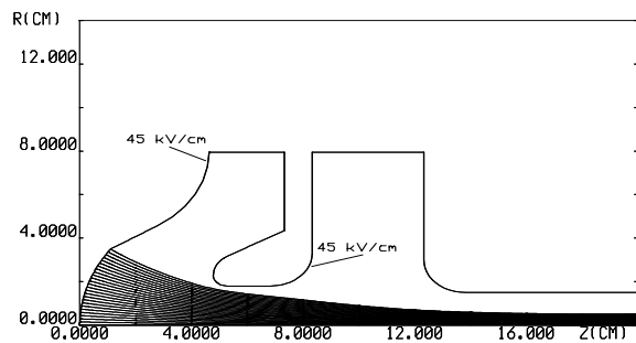
Figure 2: The gun layout and electron trajectories.
