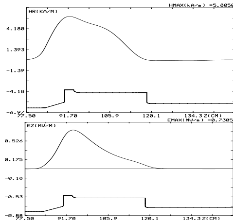
Figure 3: Profile of H and E along the cavity axis.
