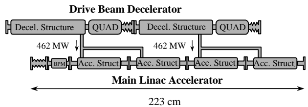
Figure 6: A module of the 3 TeV linac.
