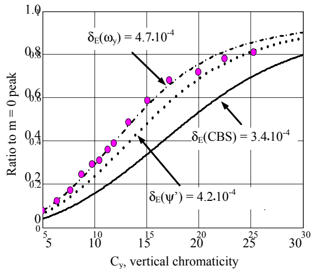
Figure 5: Ratio of R_1/R_0 for different energy spread \delta_E . Experimental points for E = 1843 \text{ MeV} are shown.
