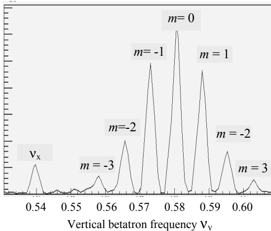
Figure 4: A spectrum of vertical betatron oscillations.
