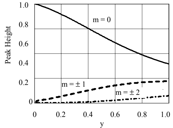
Figure 1: Relative intensities of the betatron peak and synchrotron satellites.
