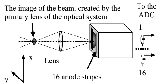
Figure 2: Optical layout of the diagnostics.
