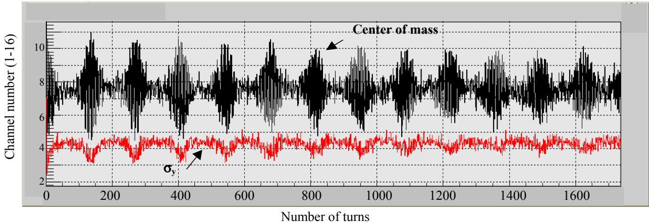
Figure 3: Beam dipole y-oscillations (upper plot) and \sigma_y behavior (down plot) after a short kick. Duration of the single turn is 1220 ns. Channel constant is 0.12 mm. I_{e^-} = 20 \mu\text{A} . C_y = 20 . E = 1843 \text{ MeV} .
