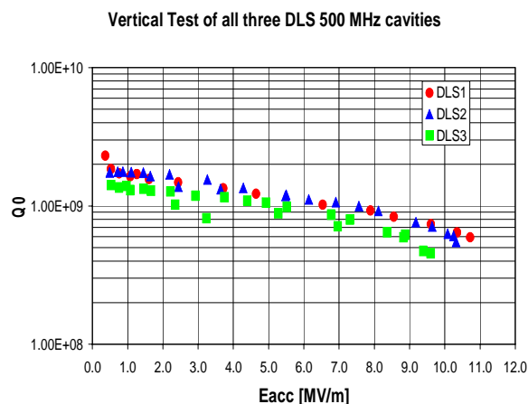
Figure 3: Results of the vertical test for each of the three cavities.
