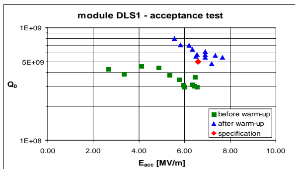
Figure 4: Q_0 of cavity 1 before and after a complete warm up and cool down.
