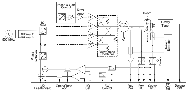
Figure 1: Schematic showing the key RF components in the RF chain
