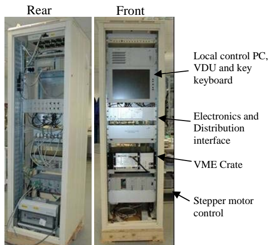
Figure 6: Front and rear view of LLRF
