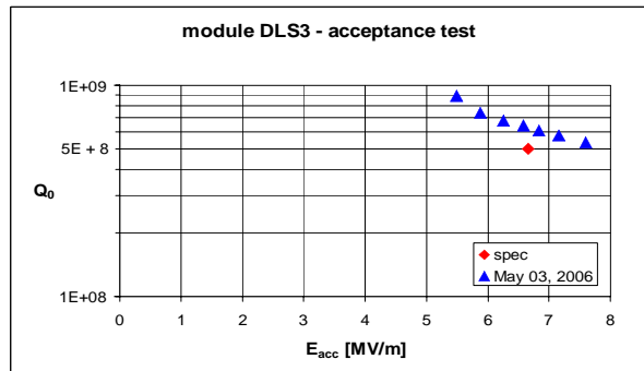
Figure 5: Q_0 of cavity 2
