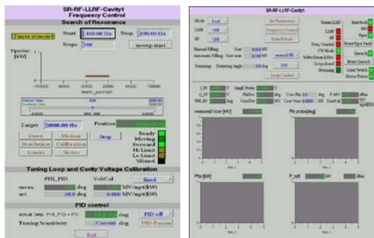
Figure 7: LLRF EPICS control screen.
