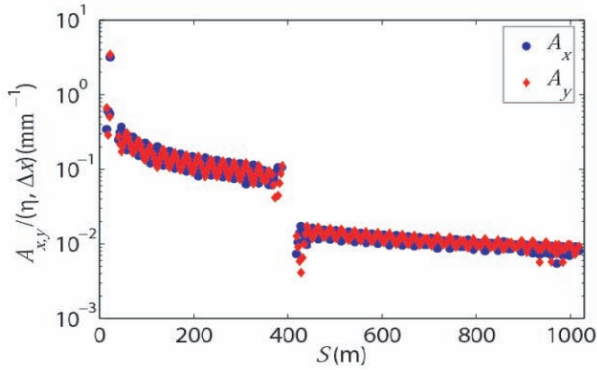
Figure 4: A_{x,y}(\eta, \Delta x) normalized to charge jitter, \eta , and cavity alignment, \Delta x , along the linac.
