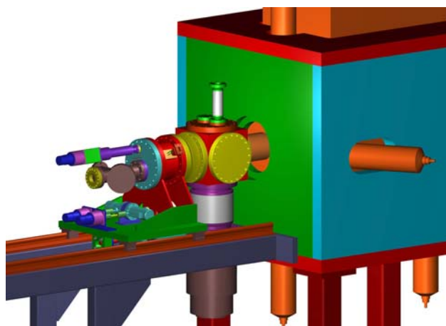
Figure 2. Injection hardware of SuSI.
