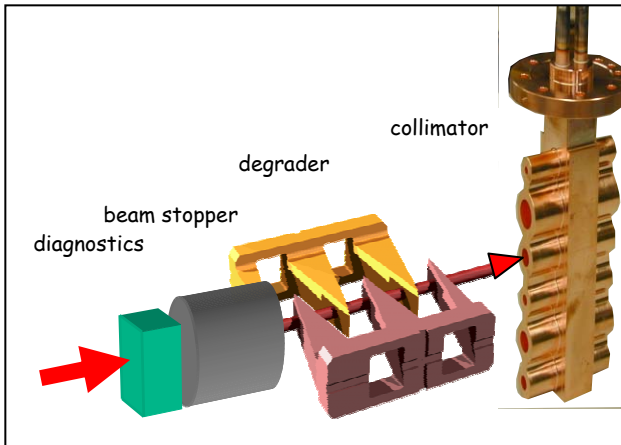
Figure 3: The degrader unit, consisting of beam diagnostics, a mechanical beam stopper, the degrader pair of multi-wedges and a collimator system.
