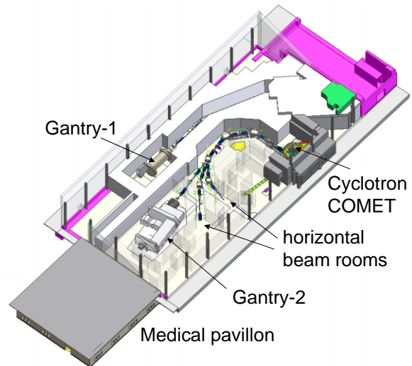
Figure 1: Layout of PSI's new dedicated proton therapy facility PROSCAN . Gantry-1 and Gantry-2 are the existing and the new gantry, respectively.
