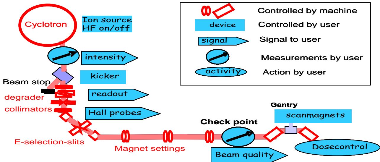
Figure 2: The separation of responsibilities between the “machine” and the “user” is an important design aspect in the PROSCAN facility.
