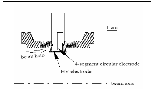
Figure 4: Sketch of the Beam-halo monitor
