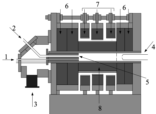
Figure 1: Schematic view of ion source. (1) gas injection (2) microwave injection (3) 150 l/sec TMP (4) extraction electrode (5) microwave tuning panel (or magnetic stainless steel cylinder + bias electrode) (6) main ring magnet (7) additional ring magnet (8) hexapole magnet
