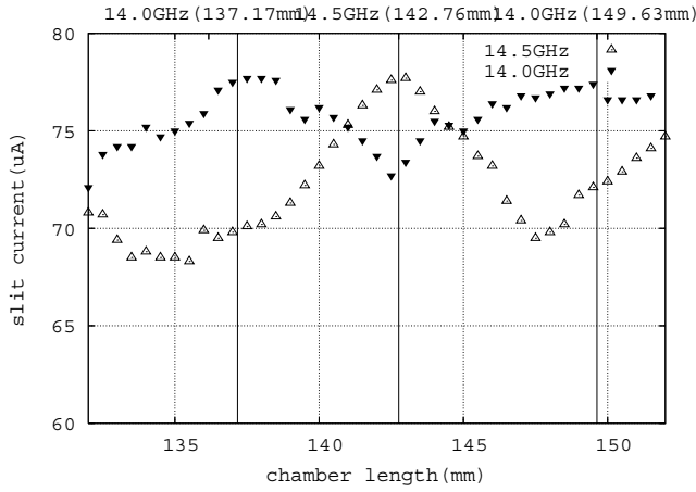
Figure 2: Dependence of the plasma chamber length for the extracted \text{Ar}^{4+} ion current with varying microwave frequency (14.0 and 14.5 GHz) of TWTA
