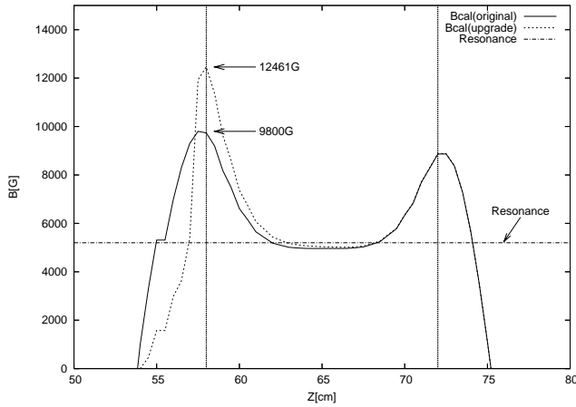
Figure 5: The calculated magnetic field distribution of axial direction in the plasma chamber using the OPERA-3D code.
