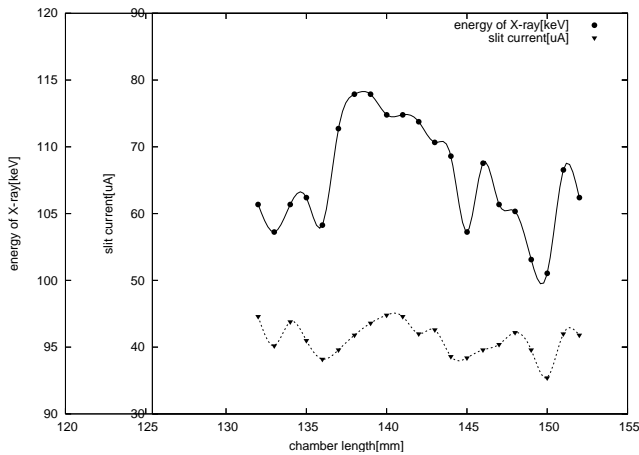
Figure 3: Dependence of extracted \text{Ar}^{8+} ion current and end-point energy of X-ray to the Plasma chamber length. Since the tuning has been for the \text{Ar}^{8+} ion extraction, this figure shows the different pattern of cavity resonator mode from fig.2.
