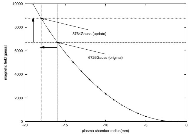
Figure 4: The calculated magnetic field distribution of radial direction in the plasma chamber using the OPERA-3D code.
